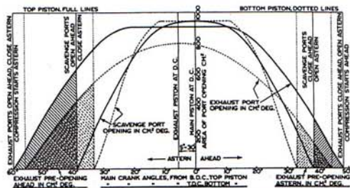
FIG. 2.—EXHAUST AND SCAVENGE PERIODS
