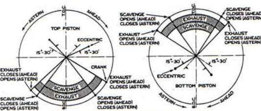
FIG. 3.—EXHAUST AND SCAVENGE PERIODS
