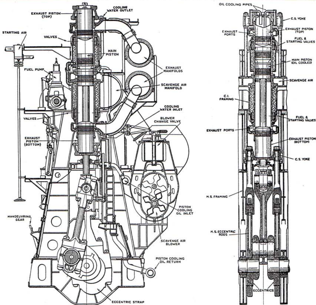
FIG. 1.—SECTIONS THROUGH HARLAND & WOLFF TWO-STROKE, DOUBLE-ACTING, OPPOSED-PISTON DIESEL ENGINE
